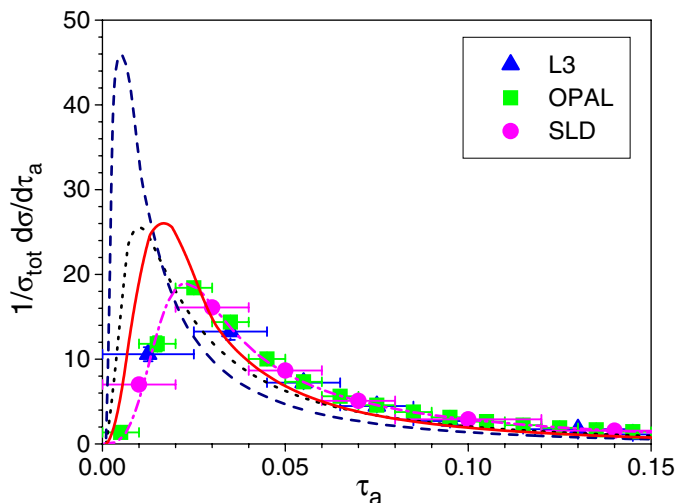
Fig. 1. Differential distributions (1/\sigma_{\text{tot}})d\sigma/d\tau_a for a = 0 , and a = -0.5 at Q = 91 GeV. Dash-dotted line: output of PYTHIA, a = 0 ; dotted line: perturbative contribution at NLL/NLO, a = 0 , as defined in (5); dashed line: same as dotted line, at a = -0.5 ; solid line: prediction for a = -0.5 using (6) and (8). The data are taken from [16]
